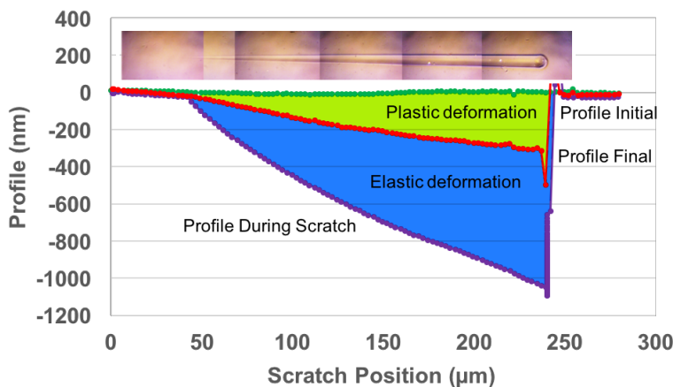
Figure 1 Scratch curves for polycarbonate. The green trace is the original morphology scan, the red trace is the residual deformation, and the purple trace is the scratch cycle. The insert is the micrograph of the full scratch length. All profiling was done at 5mN.
