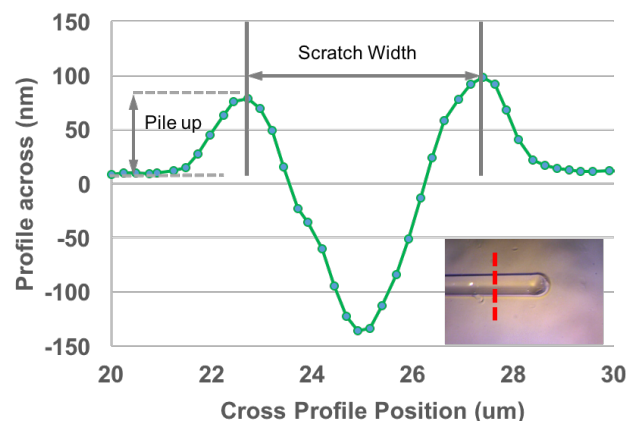
Figure 2 Profile across the scratch groove. Scratch width is defined as the peak-to-peak distance perpendicular to the scratch length. The insert shows the scratch at the location of the cross profile.
